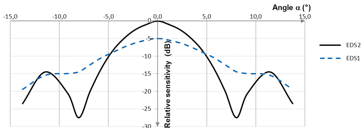
Directivity curves
